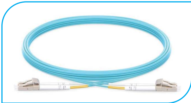
(1,2,3,5,10,15,20,25,30) M MULTI MODE LC-LC/UPC DUPLEX FIBER OPTIC PATCH CORD LSZH OM3
